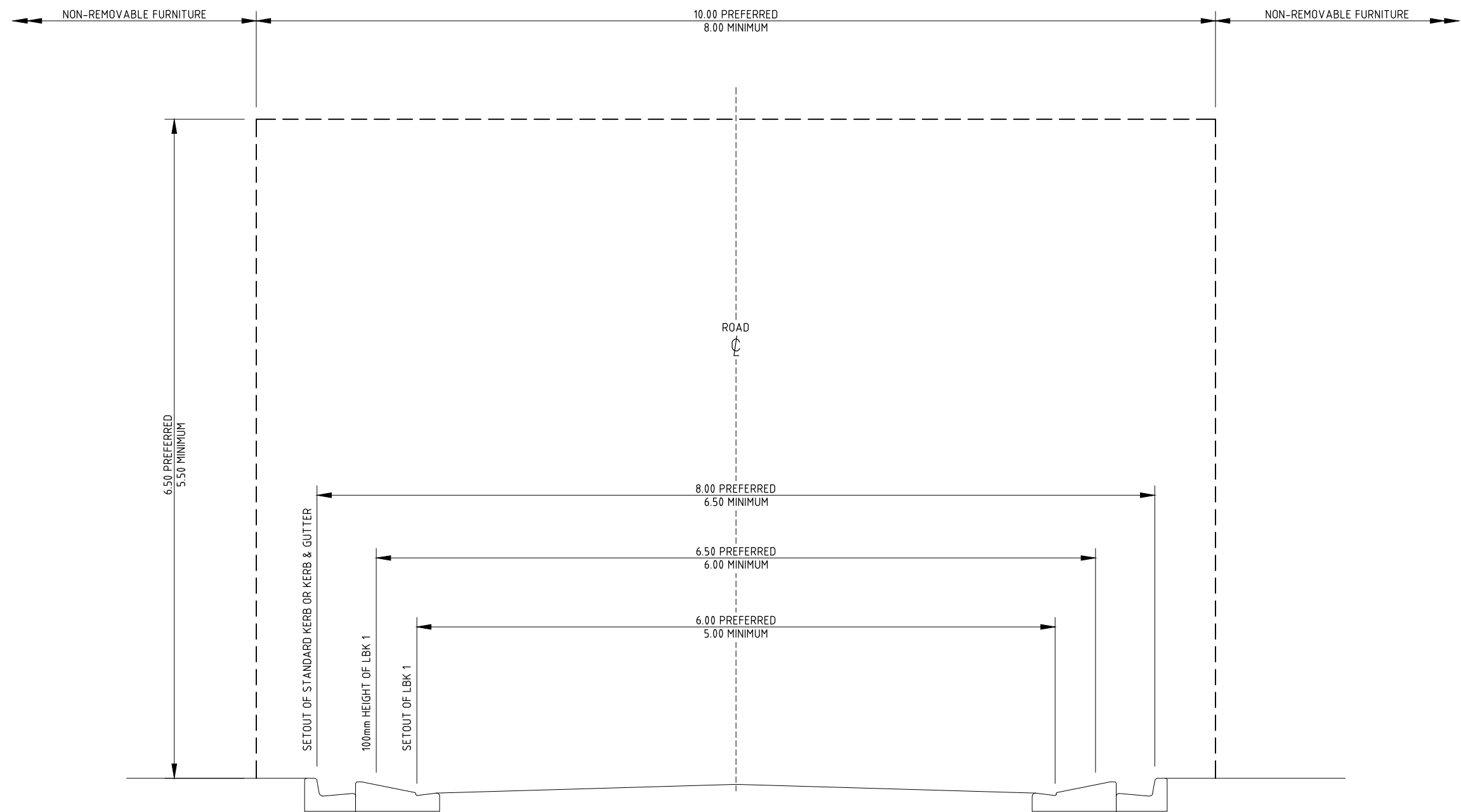
DESIGNATED "WIDE LOAD VEHICLE" CLEARANCE REQUIREMENTS NOT TO SCALE
