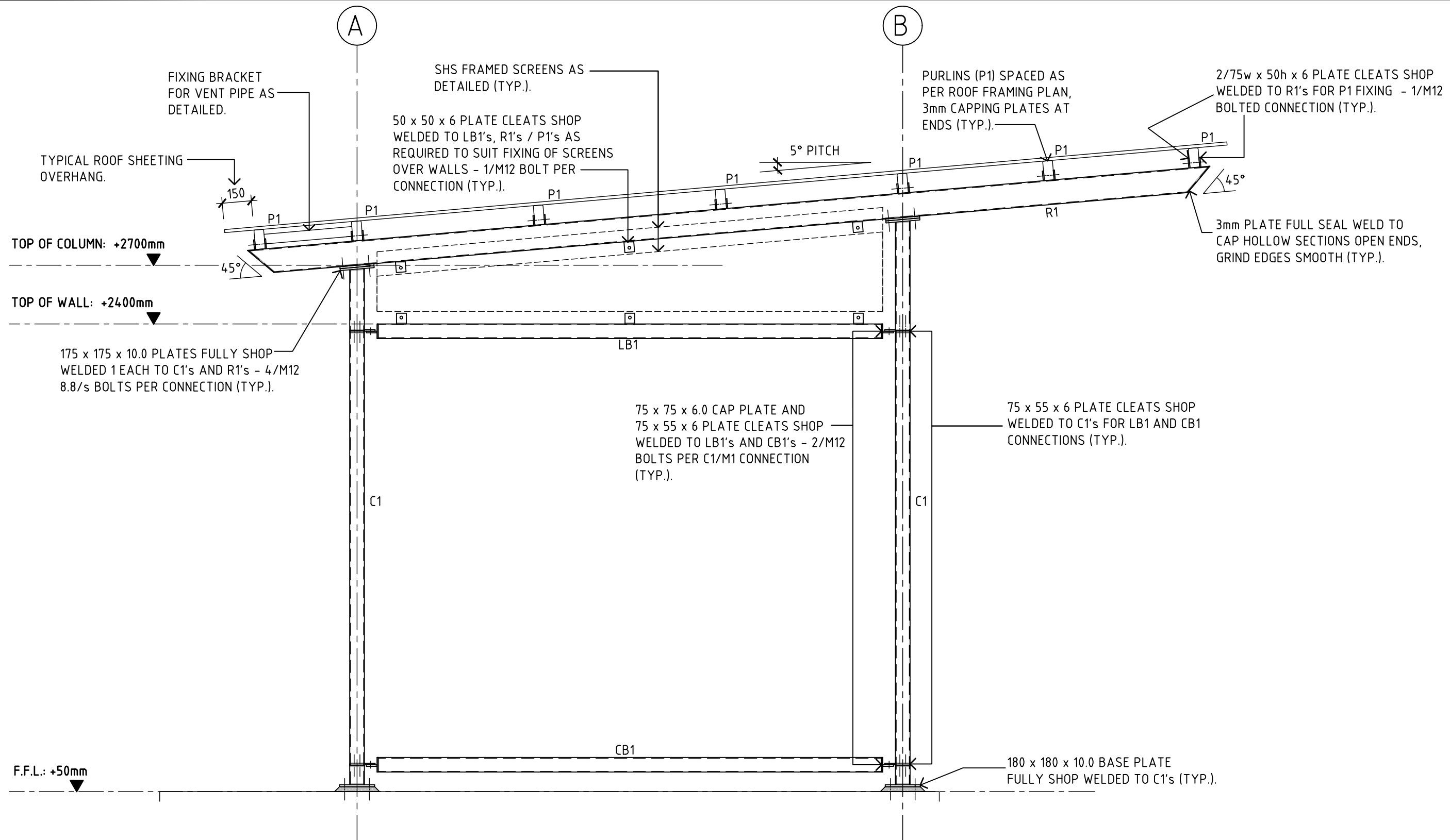
5 SECTION A09 SCALE - 1:20 0 500 1m
