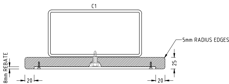
TYPICAL TIME TABLE HOLDER DETAIL
