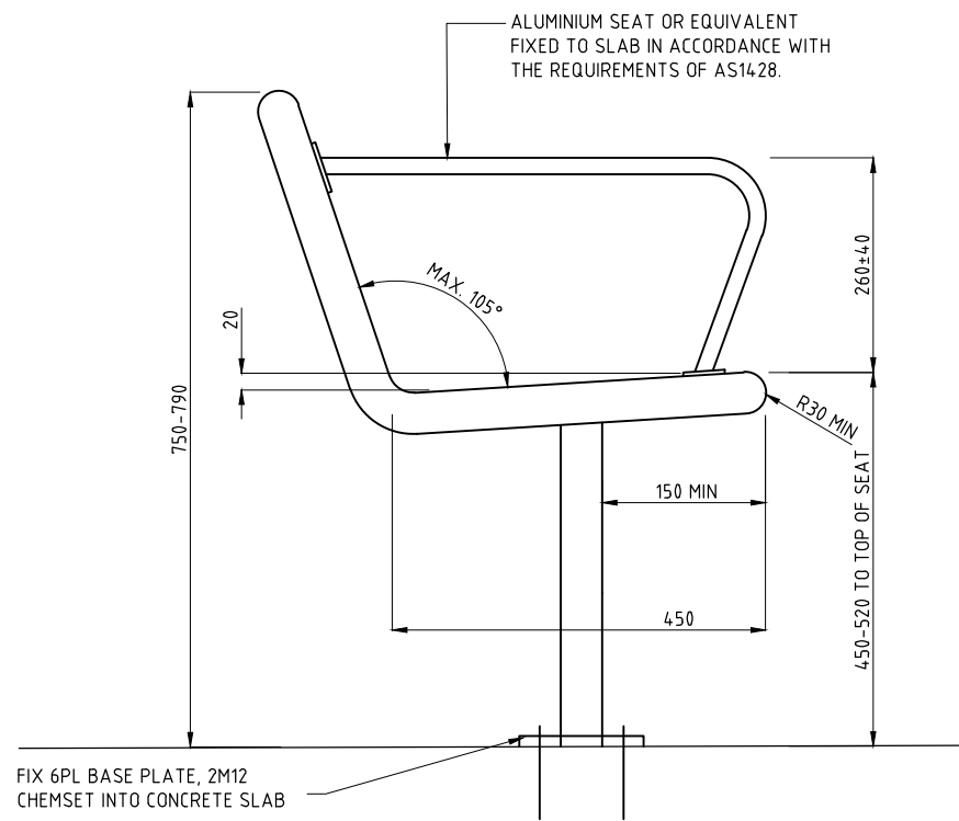
TYPICAL SEAT DETAIL
