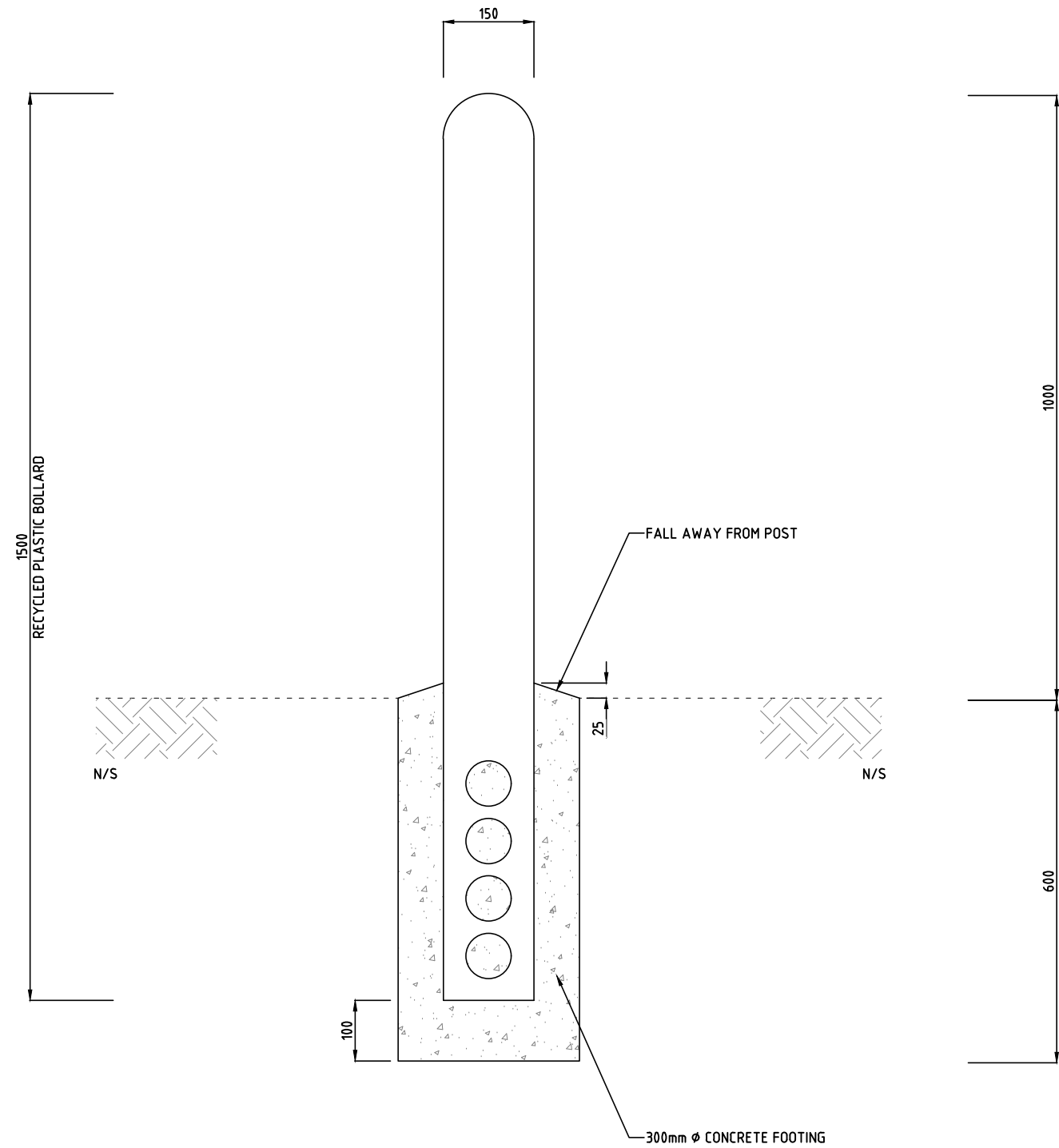
RECYCLED PLASTIC BOLLARD INSTALLATION NOT TO SCALE
