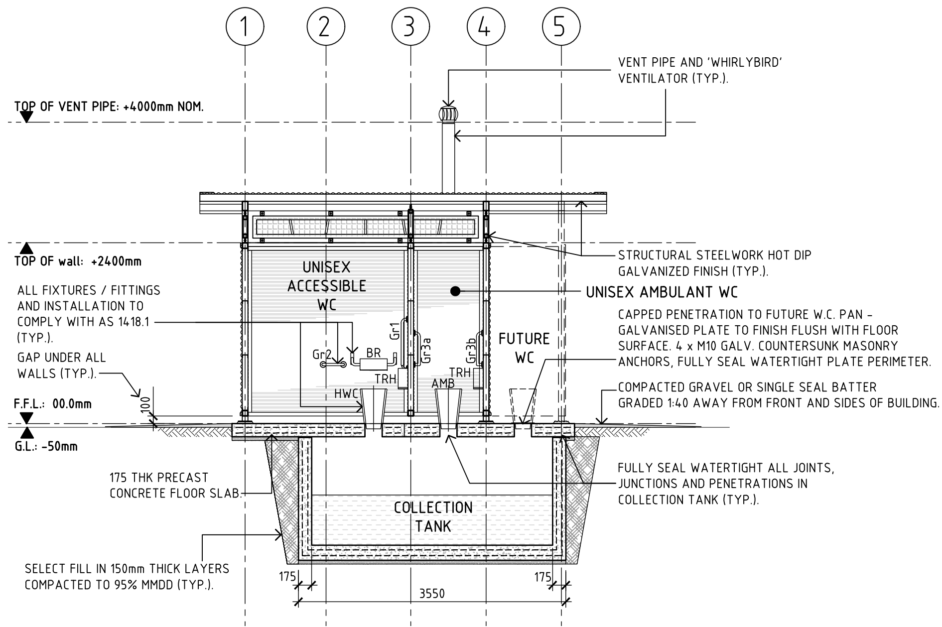
3 SECTION A01 SCALE - 1:50 0 1 2m
