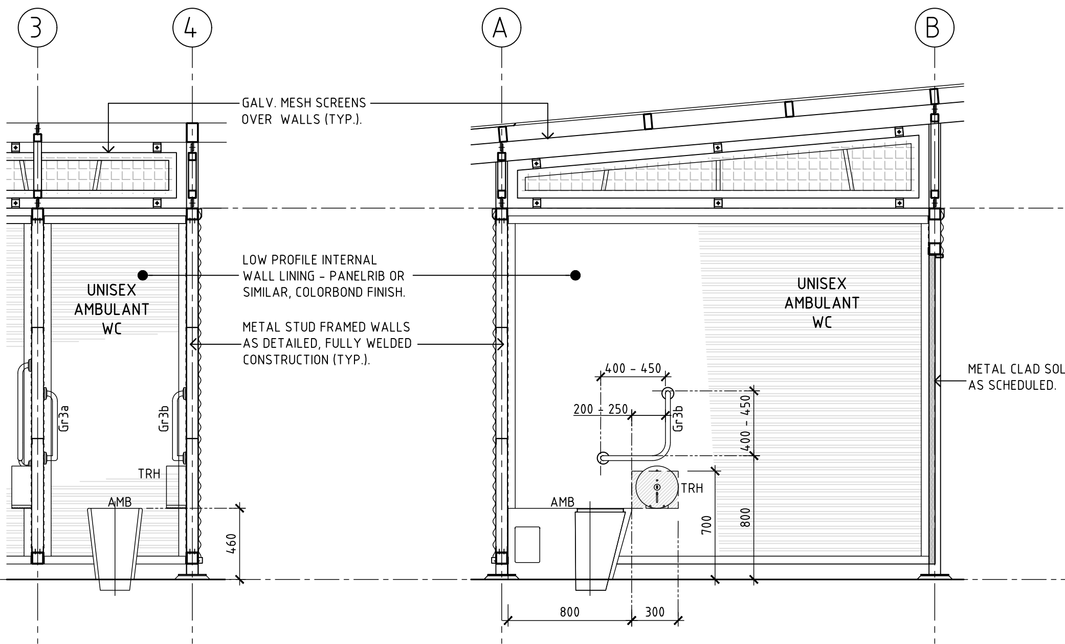
7 ELEVATION A01 SCALE - 1:25
