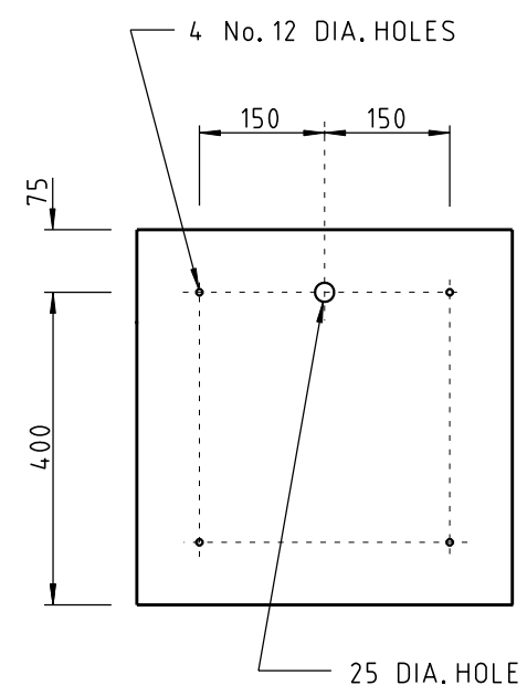
REAR ELEVATION NOT TO SCALE
