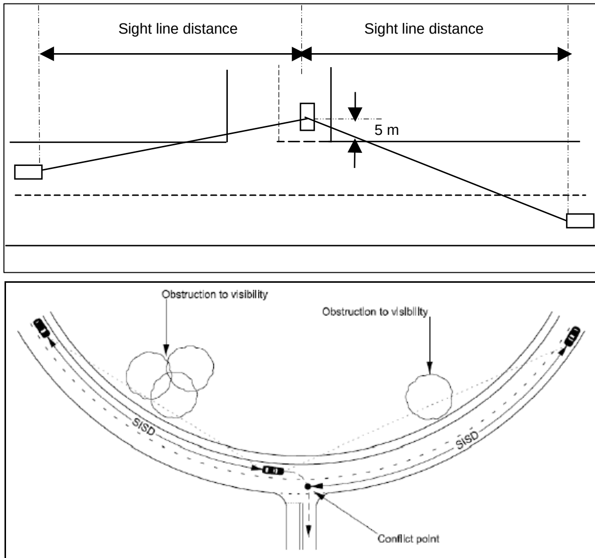
Figures - Intersection Sight Lines
